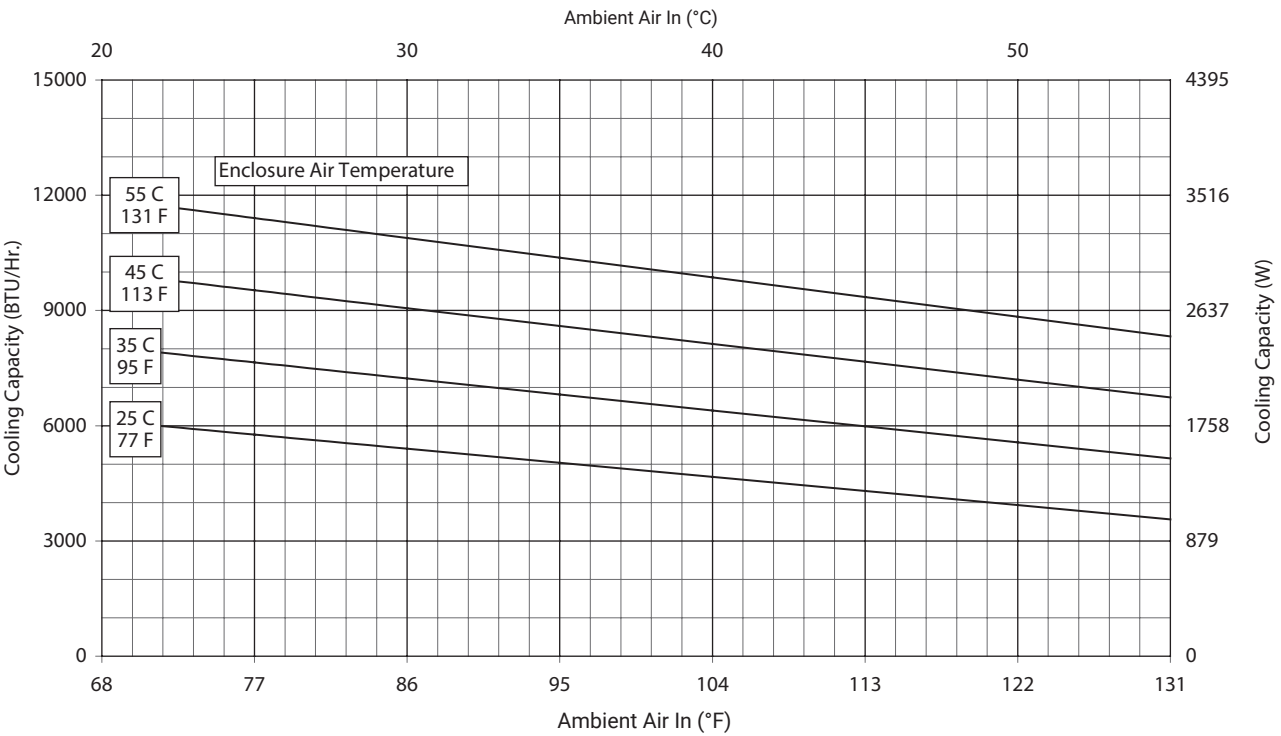
G52-0826-GXXX Capacity Curves at 60 Hz
