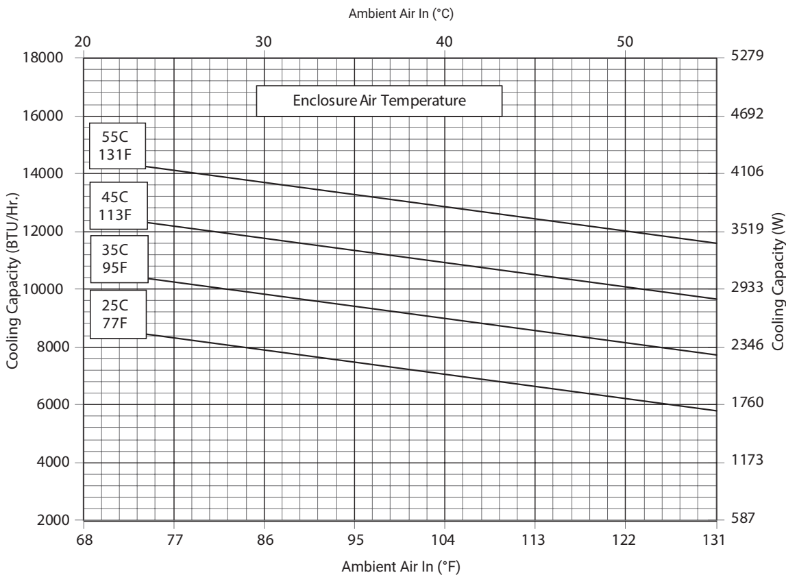
G52-1246-GXXX Capacity Curve 60 Hz
