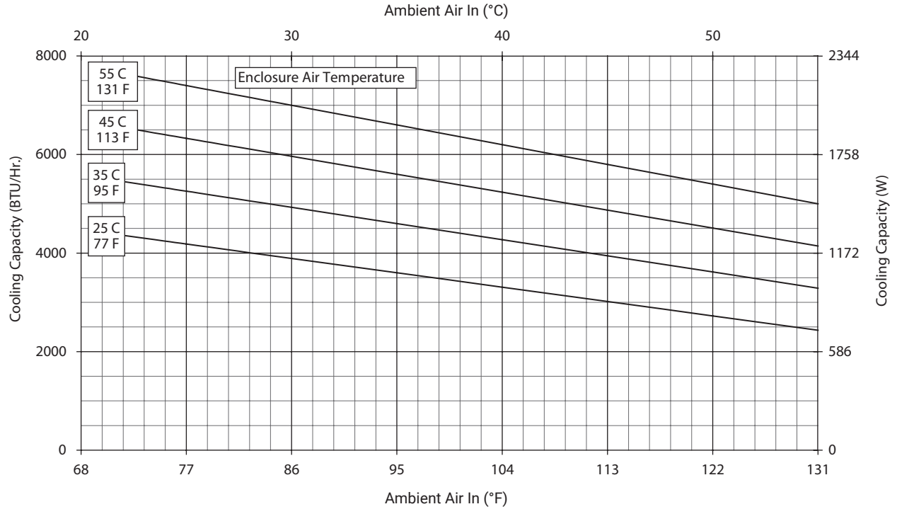
G28-0426-GXXX Capacity Curves at 60 Hz Without Air Filter
