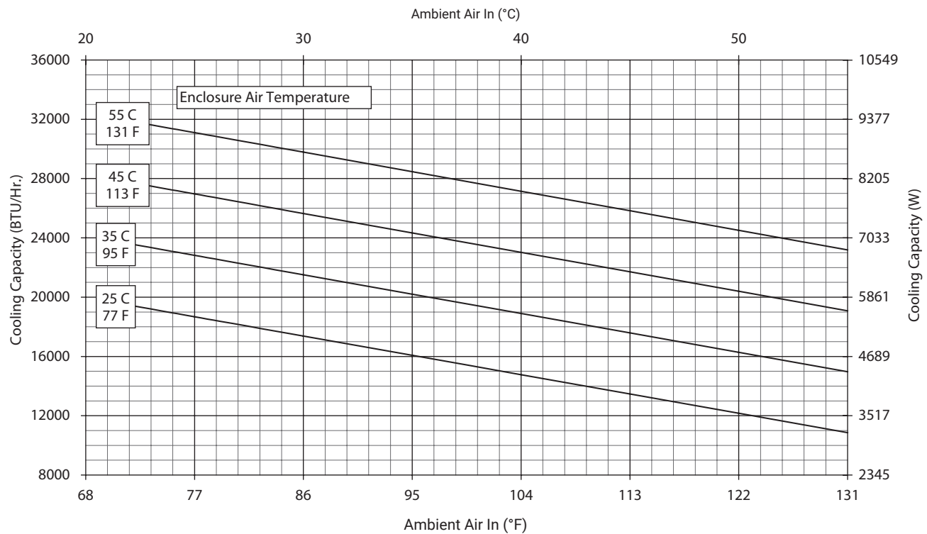
G57-2026-GXXX Capacity Curves at 60 Hz
