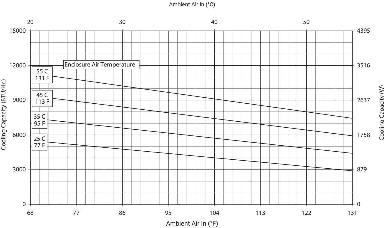
G52-0826-GXXX Capacity Curves at 50 Hz
