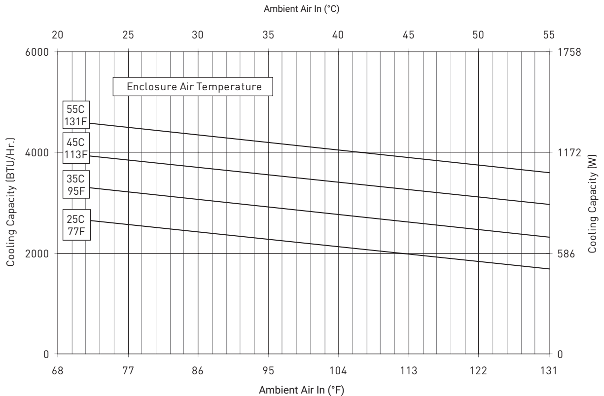
G28-0416-GXXX Capacity Curves at 50 Hz
