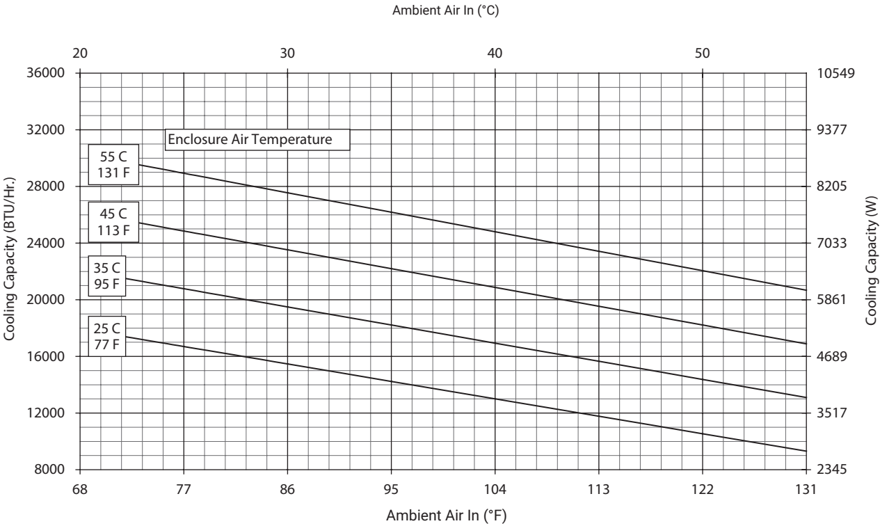
G57-2046-GXXX Capacity Curves at 50 Hz
