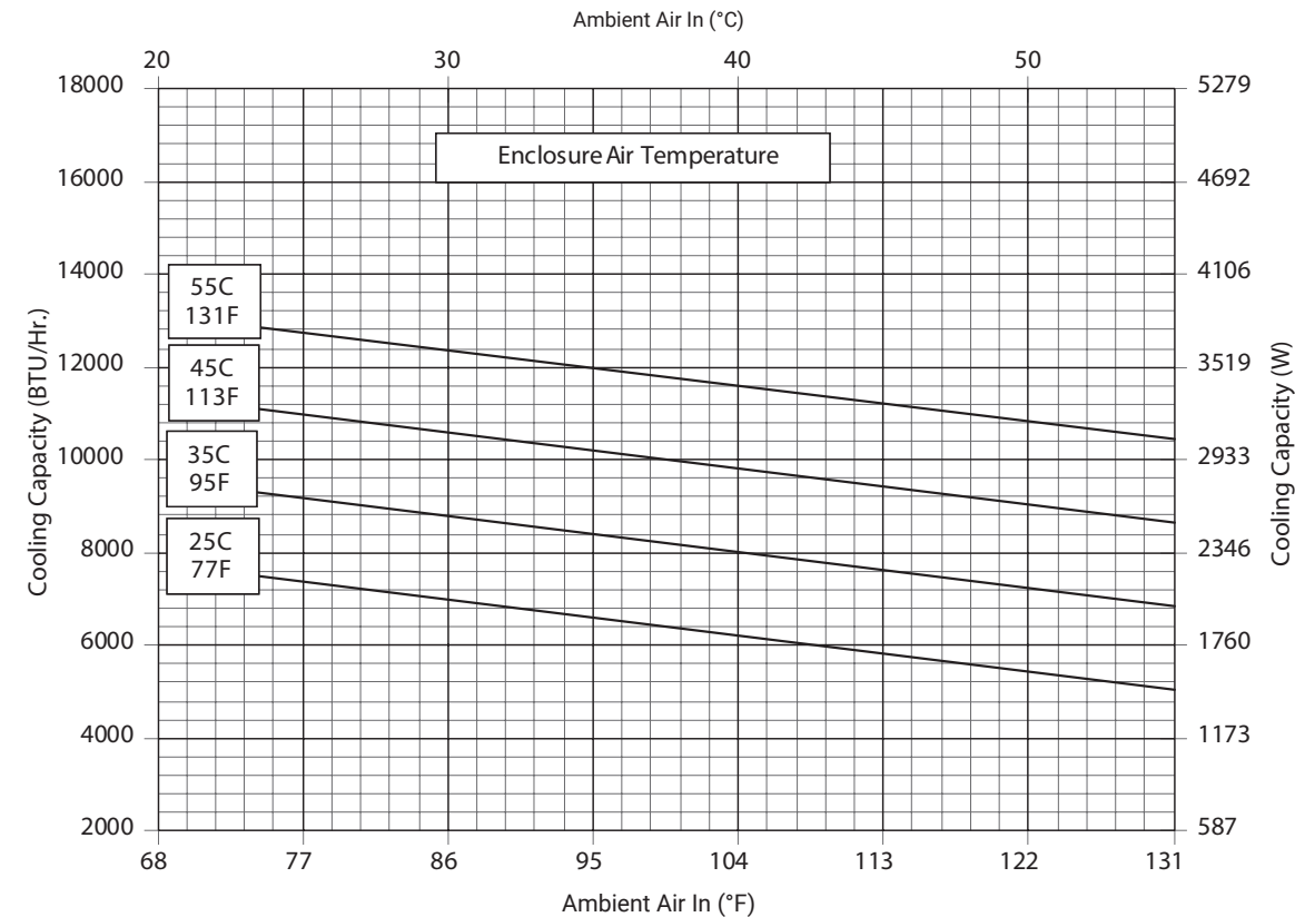
G52-1246-GXXX Capacity Curve 50 Hz
