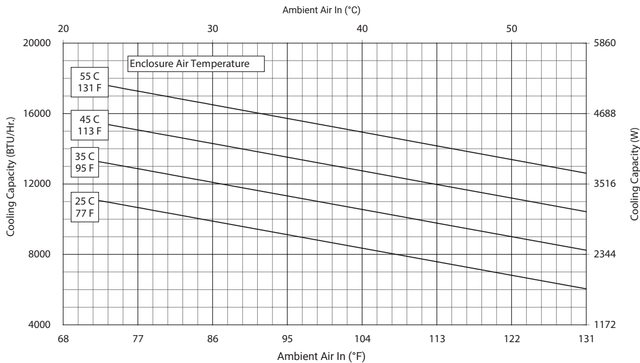
G52-1216-GXXX Capacity Curve 60 Hz
