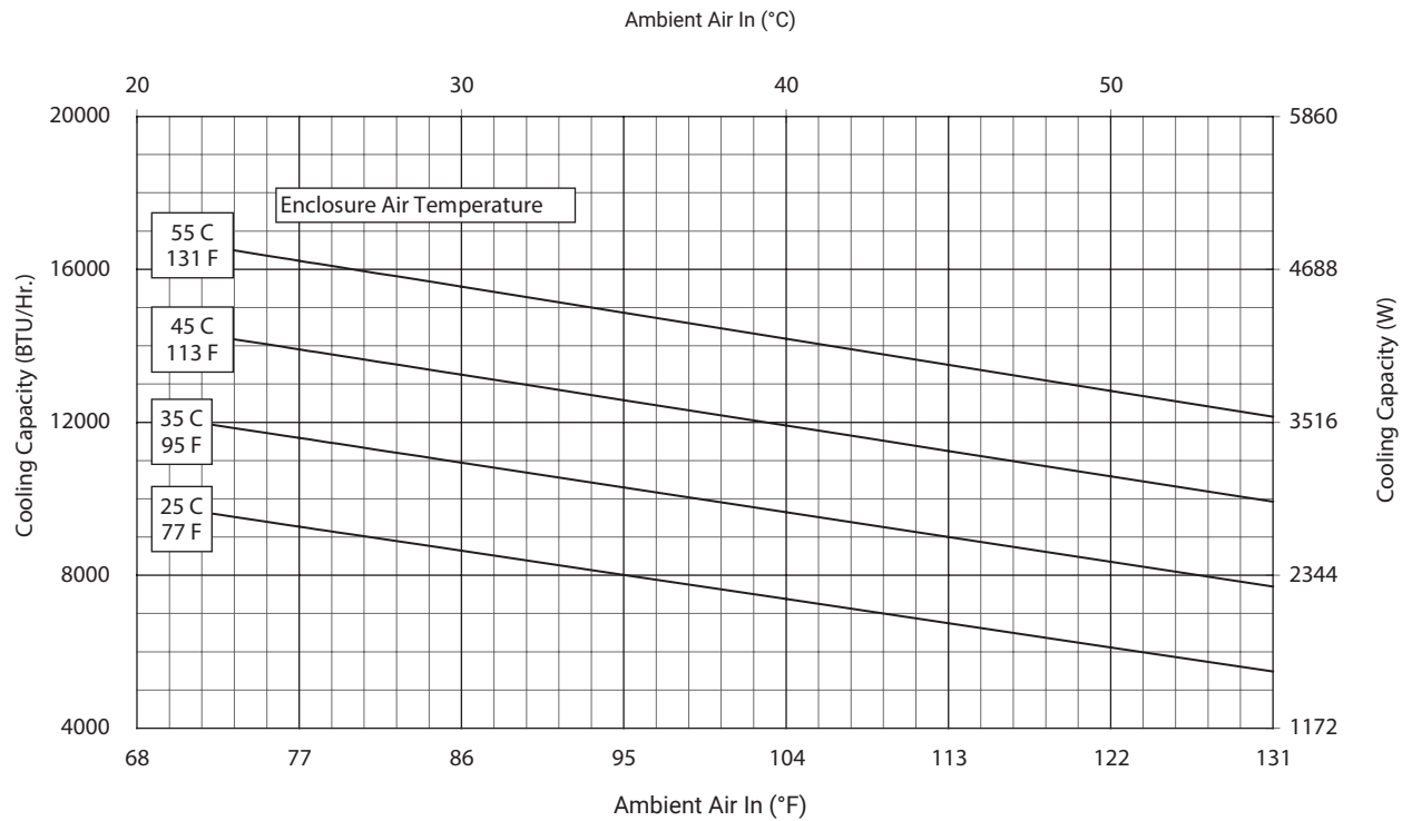
G52-1216-GXXX Capacity Curve 50 Hz
