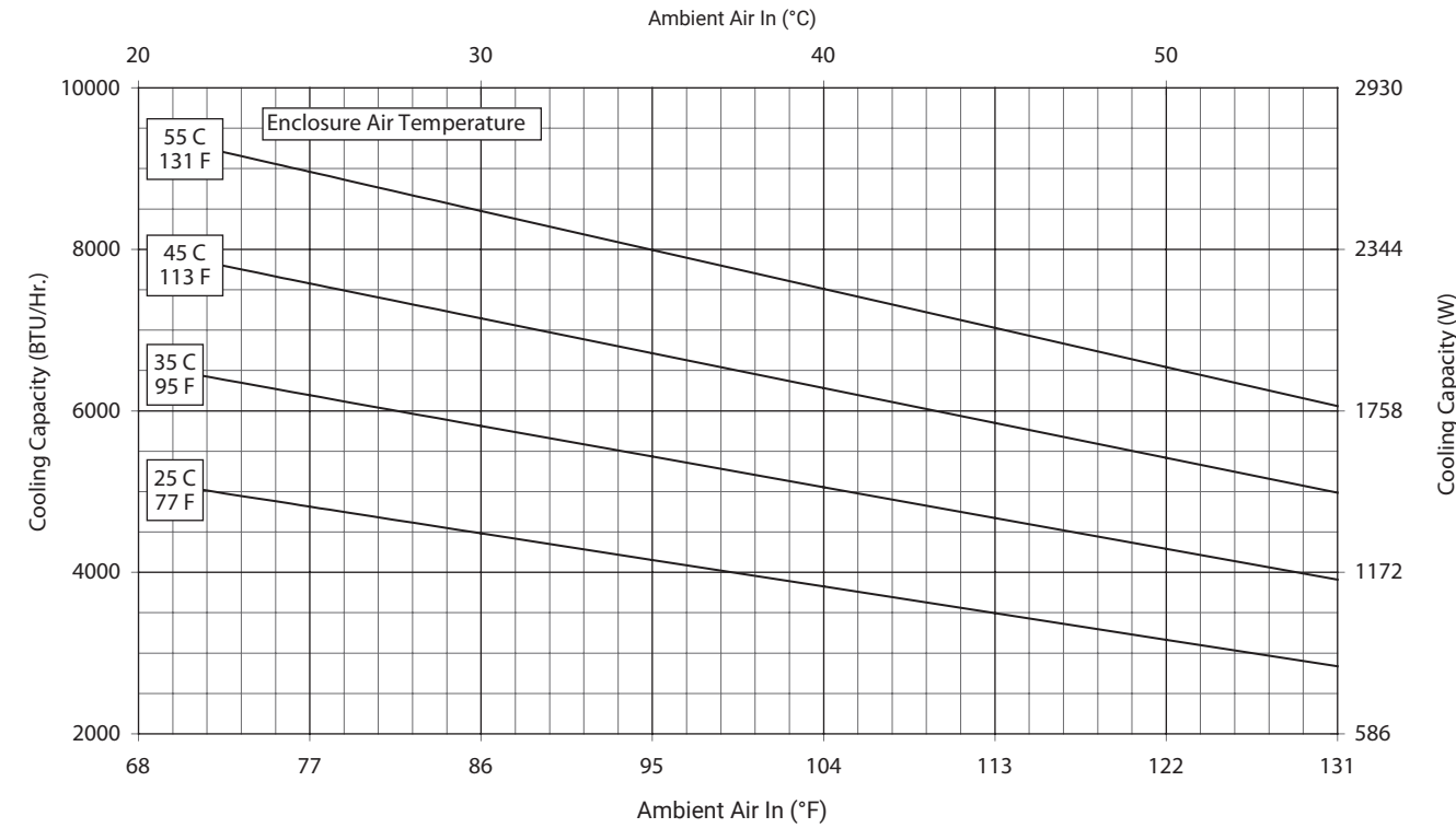
G28-0646-GXXX Performance Curve 460VAC/60Hz Without Air Filter
