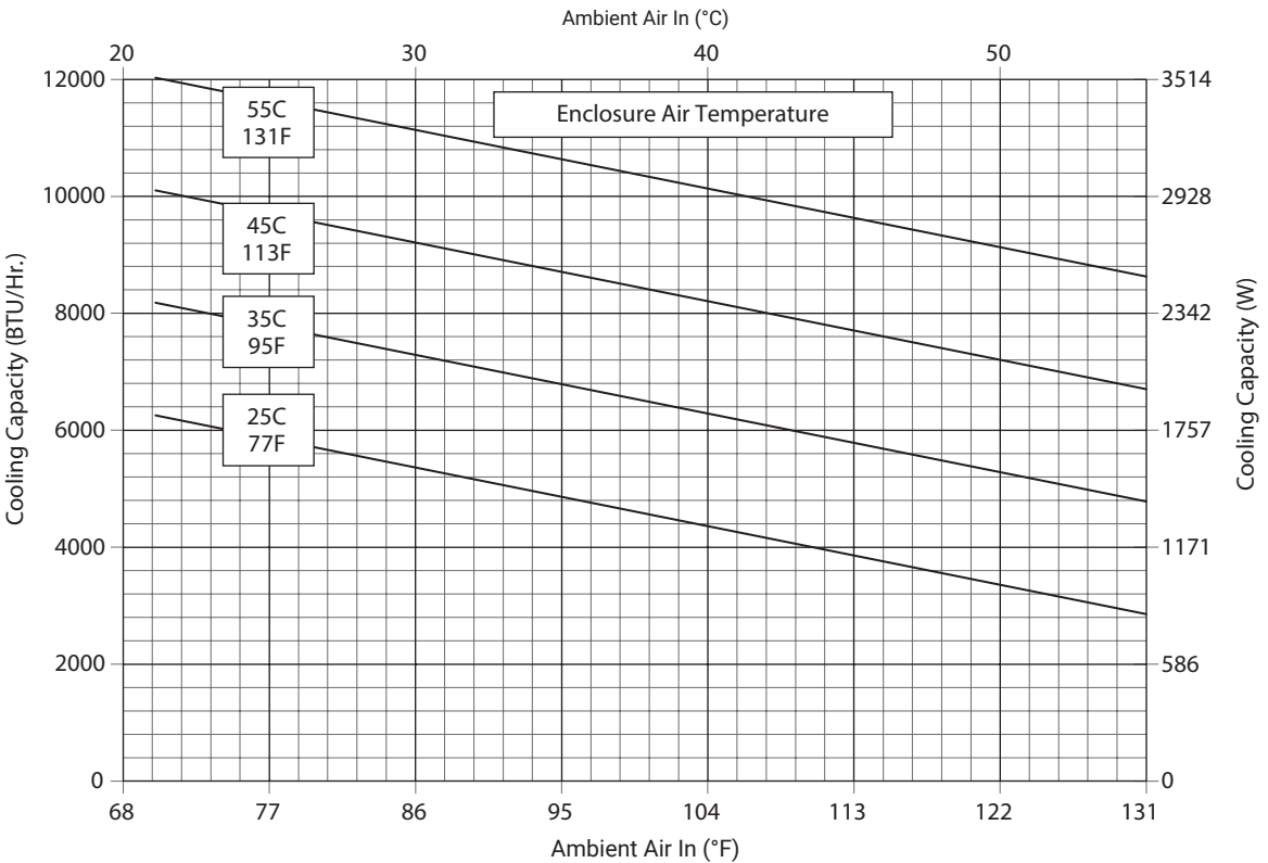
G52-0816-GXXX Capacity Curves at 60 Hz
