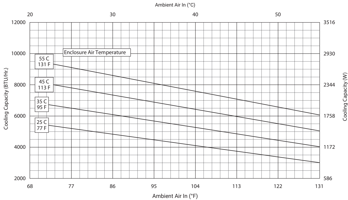
G28-06(1/2)6-GXXX Capacity Curves at 50 Hz Without Air Filter
