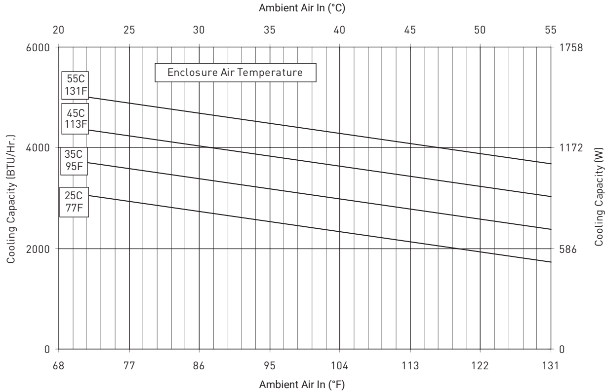
G28-0416-GXXX Capacity Curves at 60 Hz
