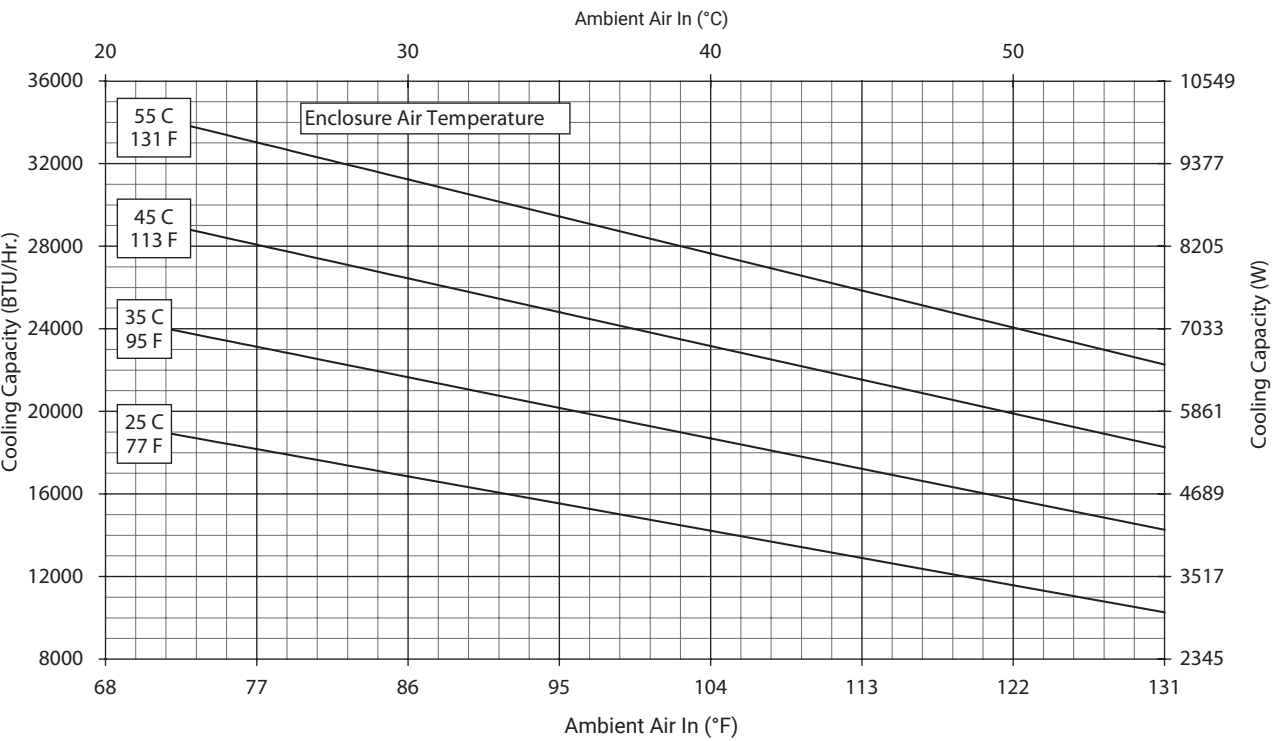
G57-2046-GXXX Capacity Curves at 60 Hz
