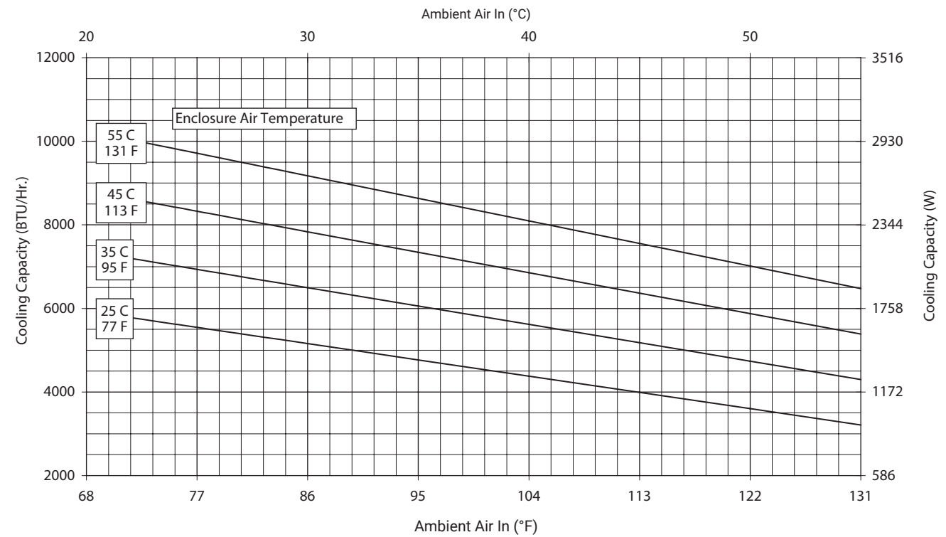
G28-06(1/2)6-G002-P#2 Capacity Curves at 60 Hz Without Air Filter
