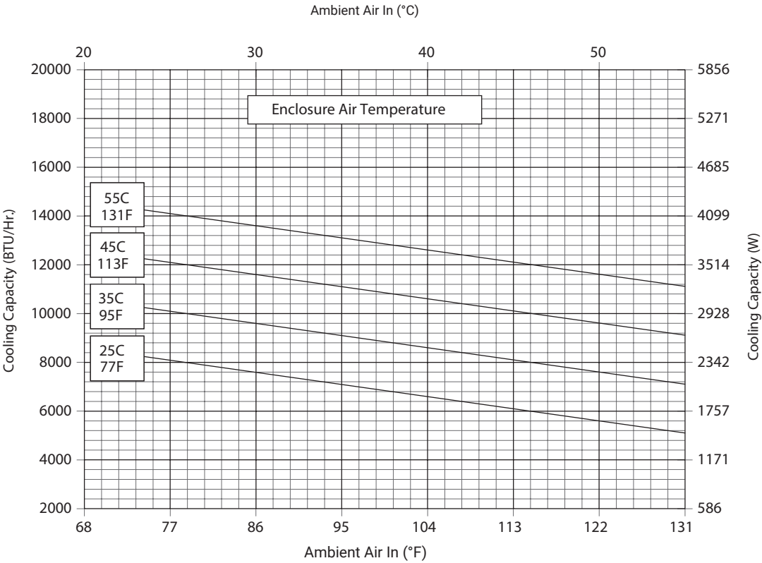
G52-1226-GXXX Capacity Curve 50 Hz
