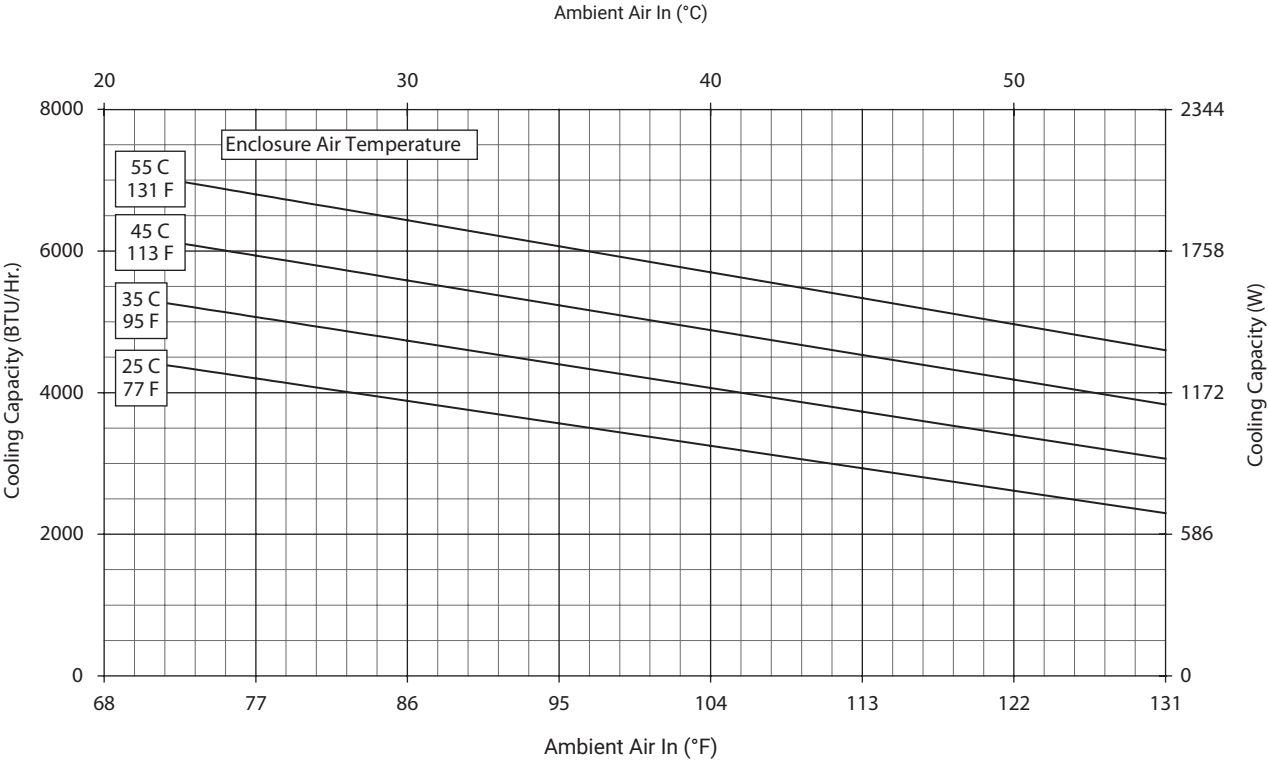
G28-0426-GXXX Capacity Curves at 50 Hz Without Air Filter
