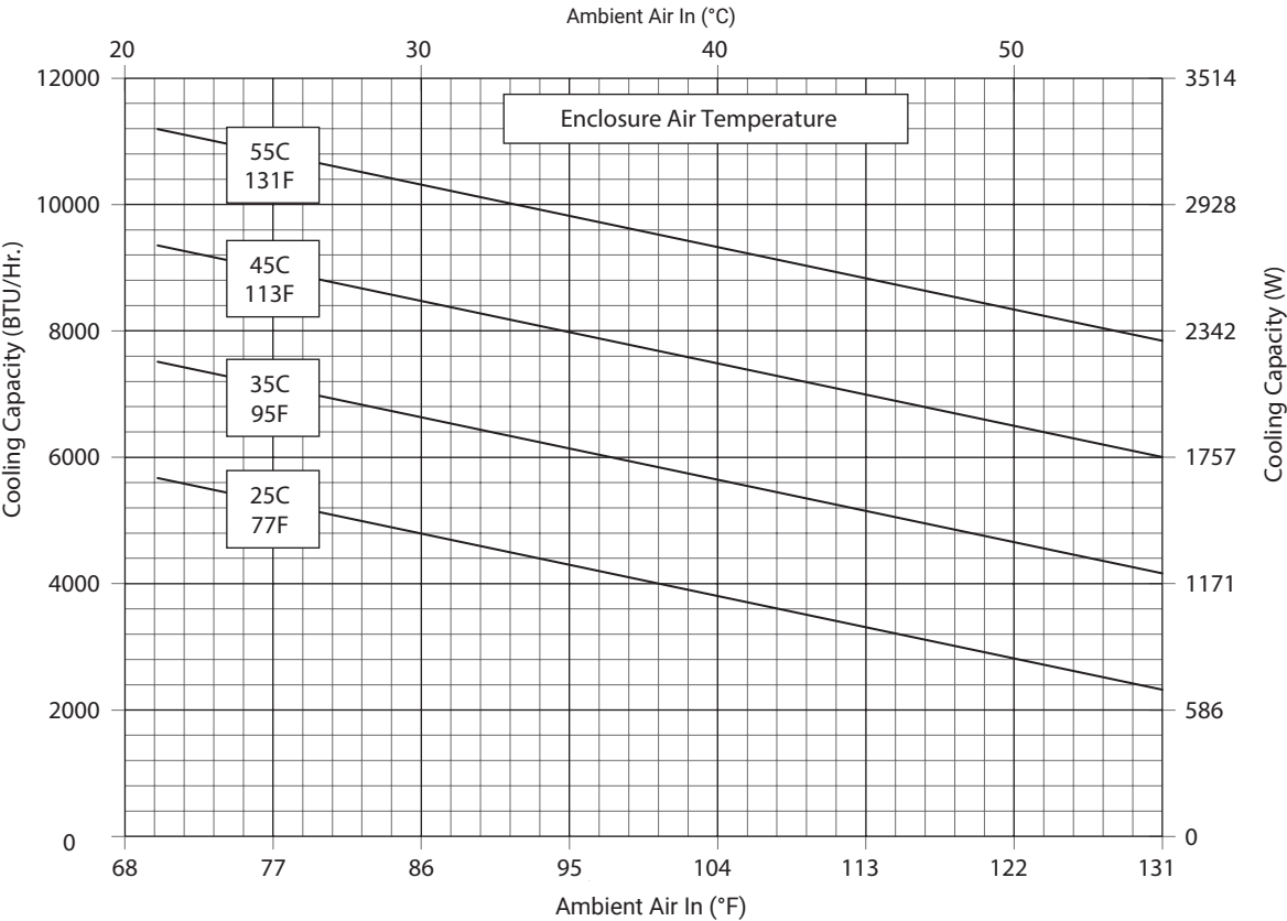
G52-0816-GXXX Capacity Curves at 50 Hz
