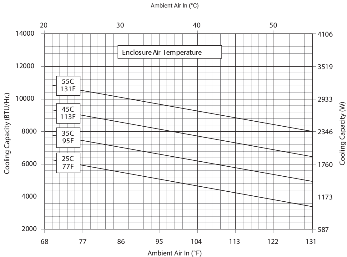
G52-0846-GXXX Capacity Curves at 50 Hz
