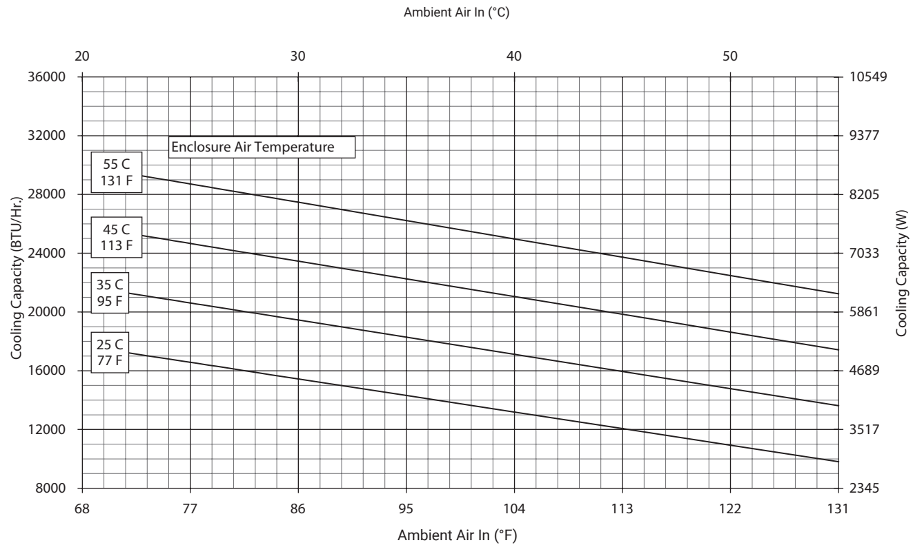
G57-2026-GXXX Capacity Curves at 50 Hz
