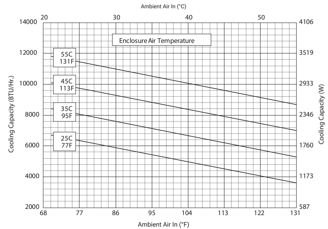
G52-0846-GXXX Capacity Curves at 60 Hz
