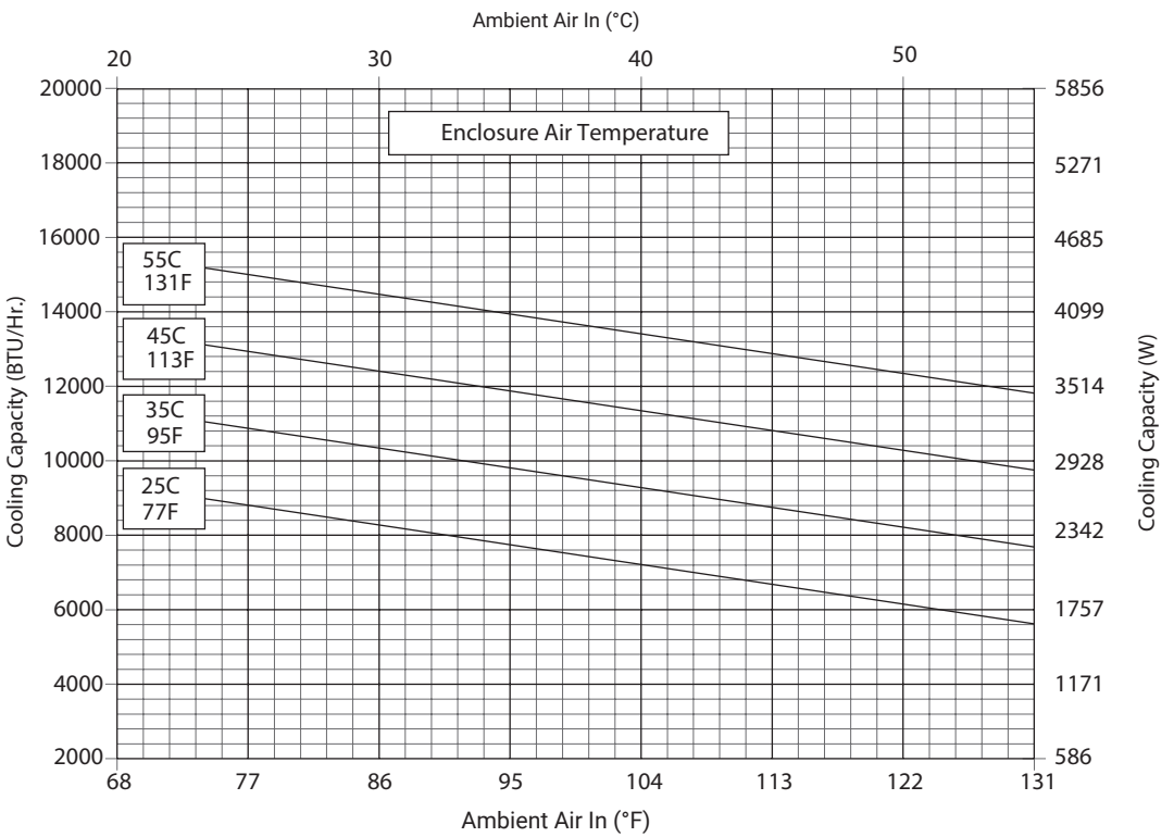
G52-1226-GXXX Capacity Curve 60 Hz
