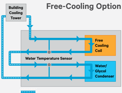
Field-supplied piping
