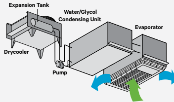
Remote Water/Glycol-Condensing Unit Supply & Return Air Plenum
