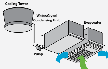
Remote Water/Glycol-Condensing Unit Supply & Return Air Plenum
